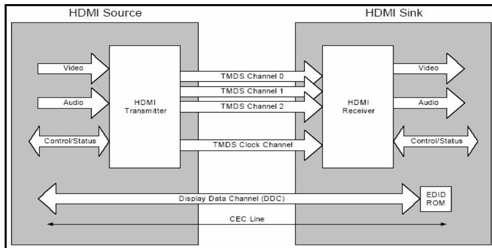
Figure 5: HDMI Link Block Diagram (Source: HDMI 1.2 Specification)
