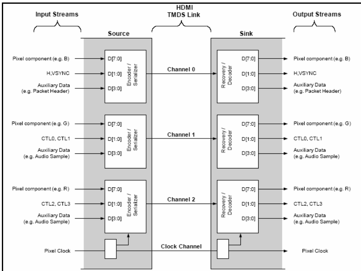
Figure 6: HDMI Link Architecture (Source: HDMI 1.2 Specification)
